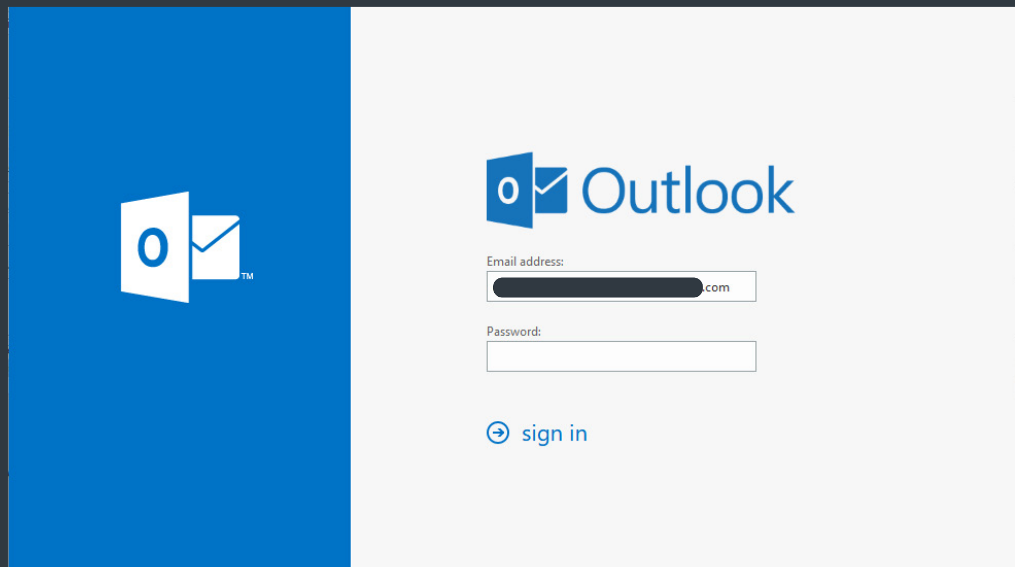
Phishing form impersonating Outlook, detected as HTML/Phishing.Outlook
